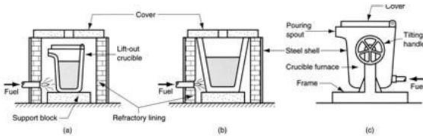
Three types: (a) lift-out crucible, (b) stationary pot, from which molten metal must be ladle (c) tilting-pot furnace
